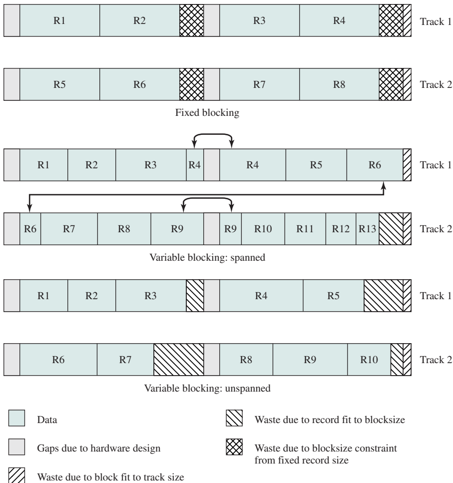
Figure 12.8 Record Blocking Methods [WIED87]
