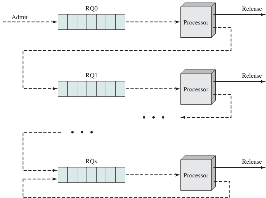
Figure 9.10 Feedback Scheduling
