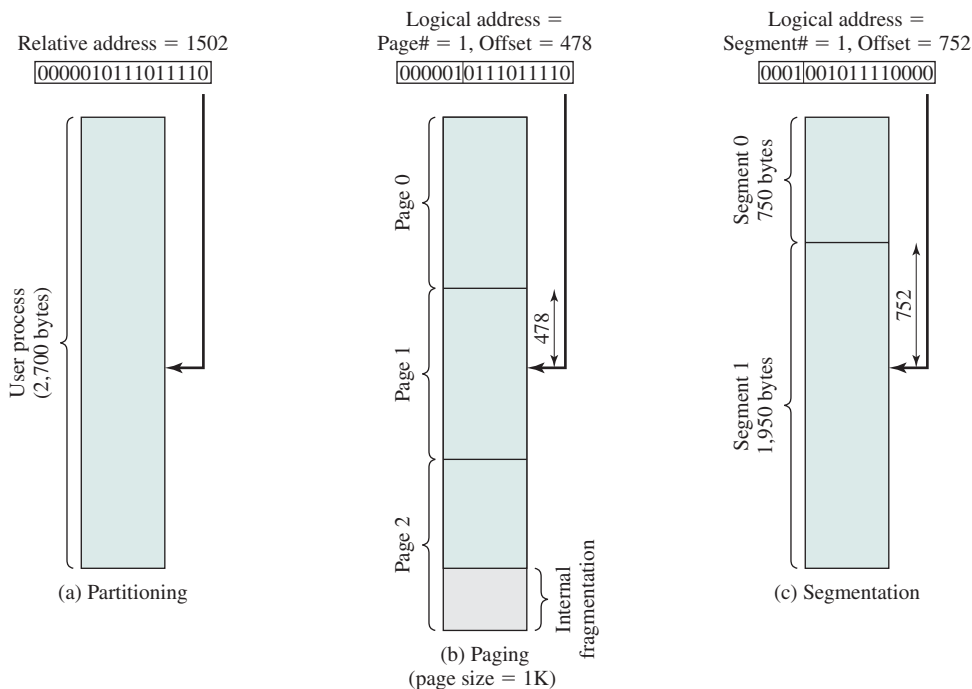
Figure 7.11 Logical Addresses
