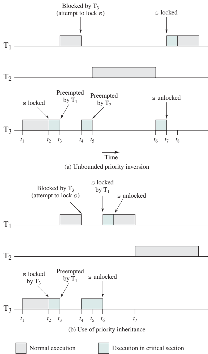
Figure 10.9 Priority Inversion
