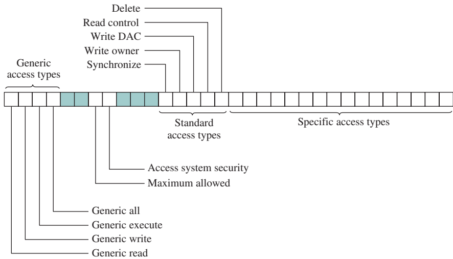
Figure 15.12 Access Mask
