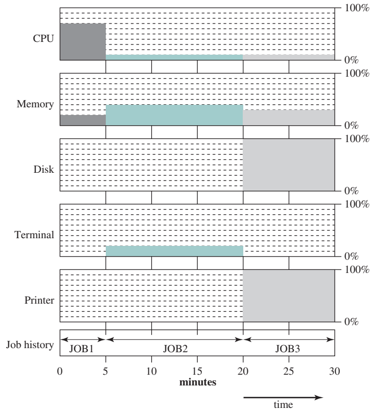
(a) Uniprogramming
