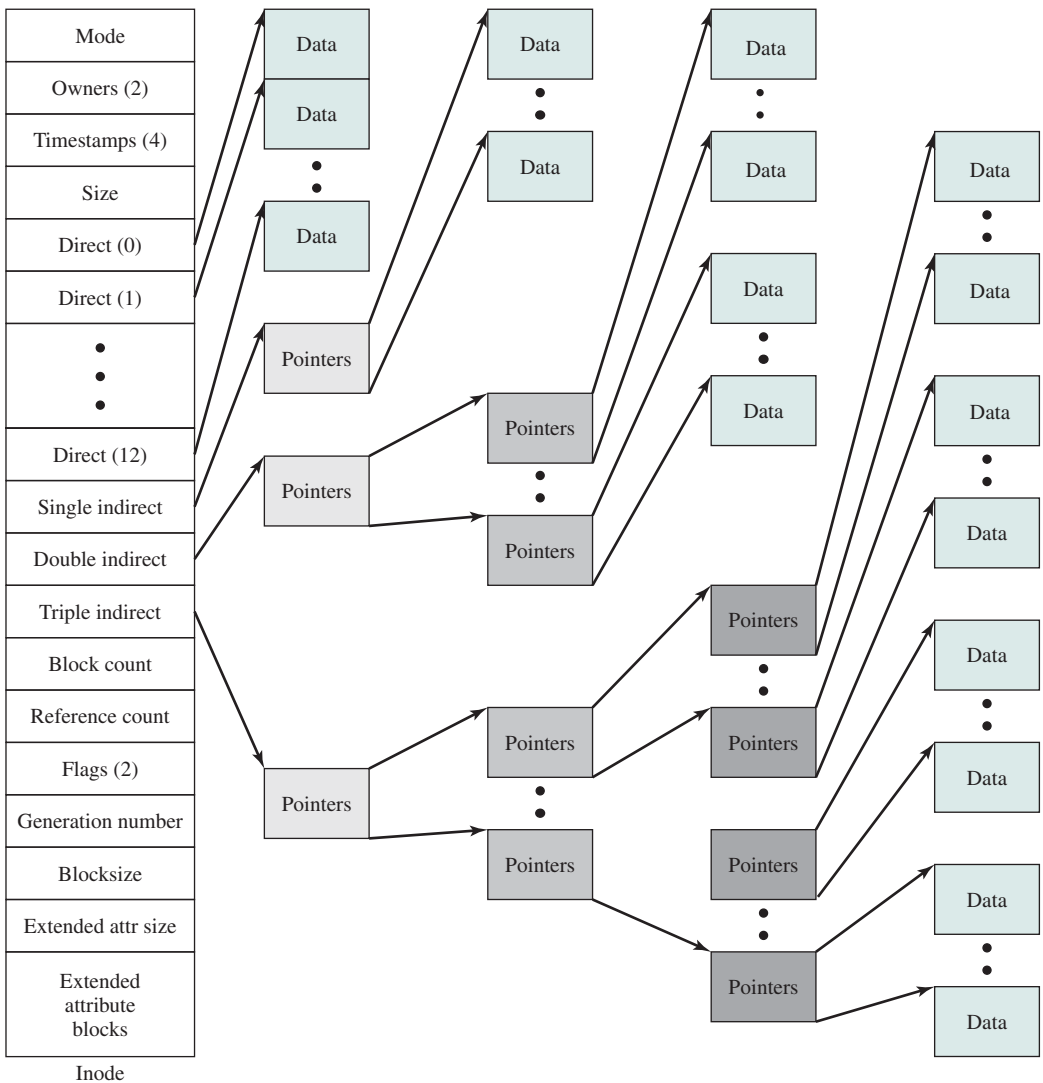
Figure 12.16 Structure of FreeBSD Inode and File
