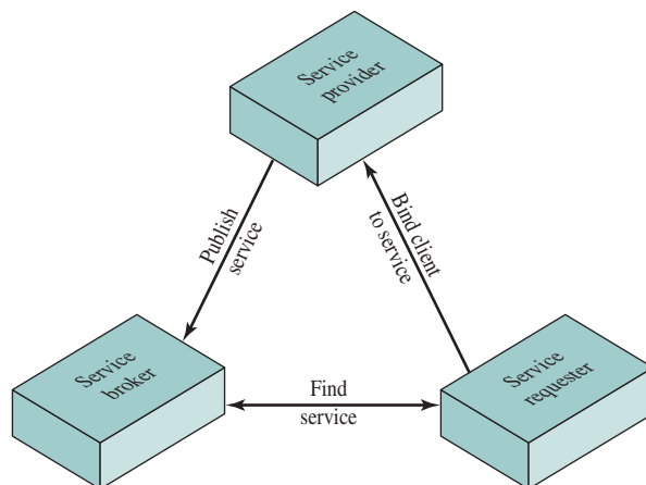
Figure 16.10 SOA Model
