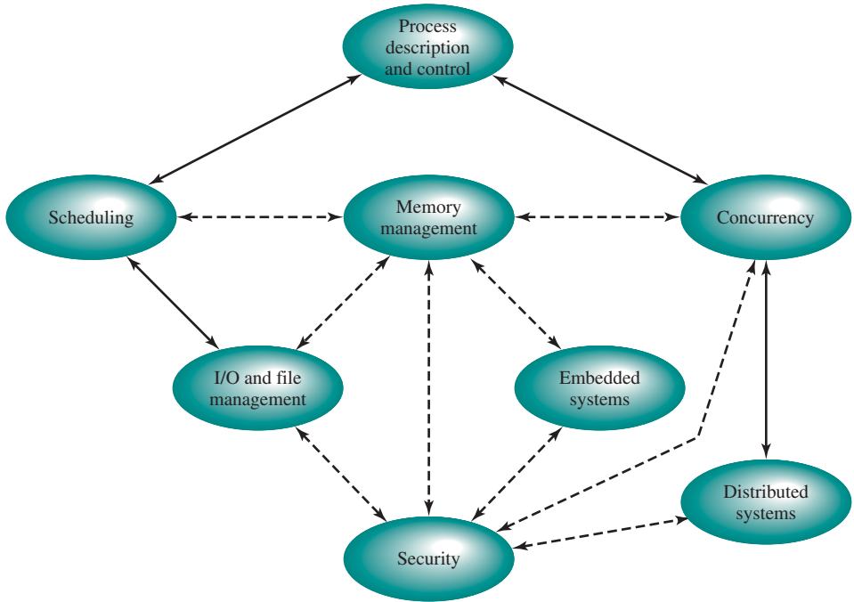
Figure 0.1 OS Topics
