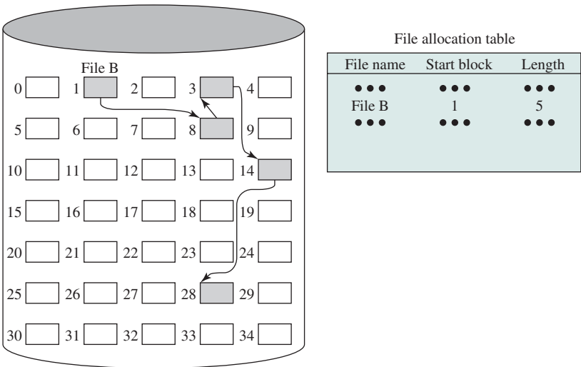
Figure 12.11 Chained Allocation
