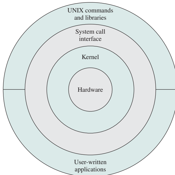
Figure 2.16 General UNIX Architecture
