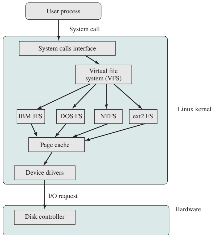
Figure 12.19 Linux Virtual File System Context
