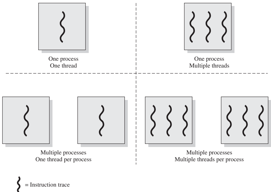
Figure 4.1 Threads and Processes [ANDE97]
