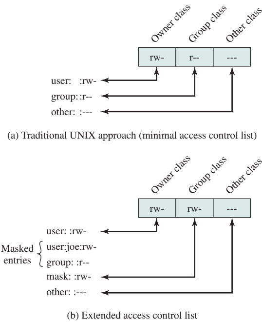
Figure 12.18 UNIX File Access Control
