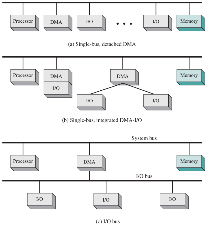
Figure 11.3 Alternative DMA Configurations
