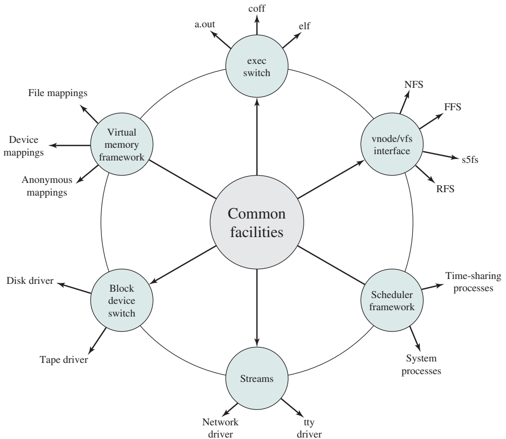
Figure 2.18 Modern UNIX Kernel
