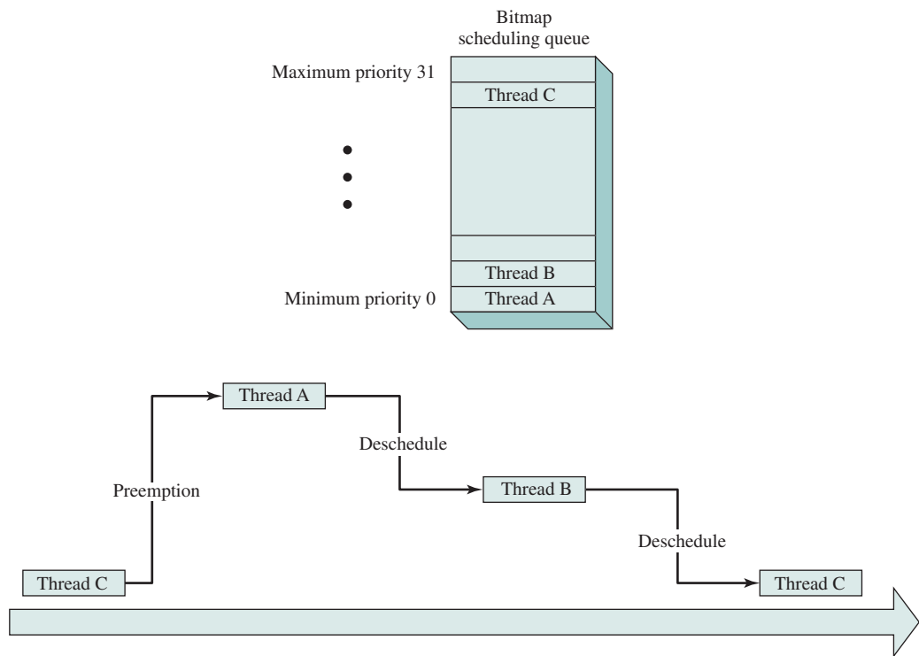
(a) Bitmap scheduler thread operation
