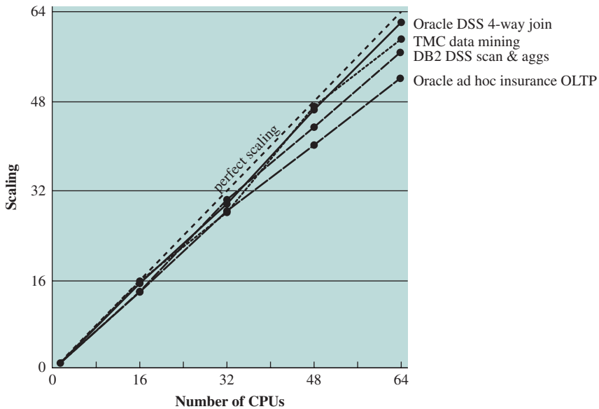
Figure 4.8 Scaling of Database Workloads on Multiple-Processor Hardware
