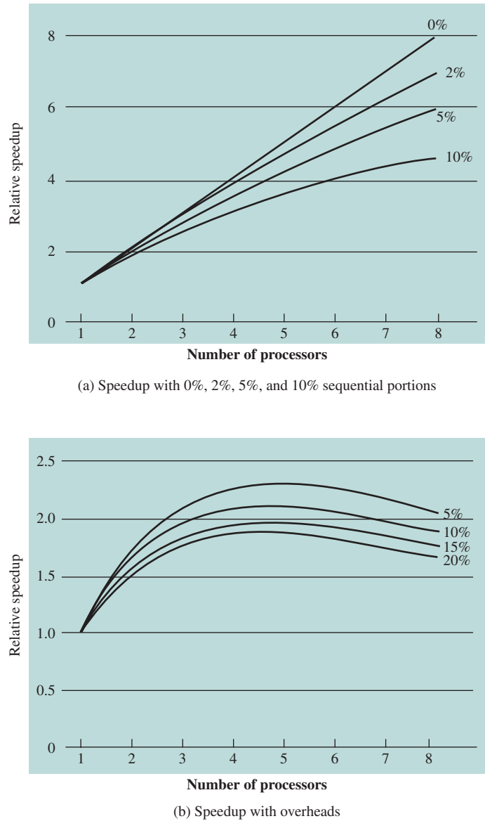
Figure 4.7 Performance Effect of Multiple Cores
