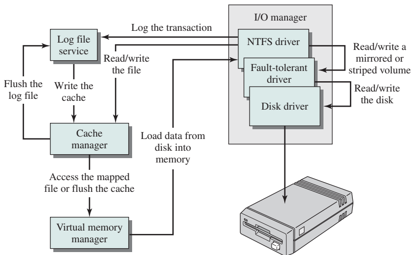
Figure 12.22 Windows NTFS Components
