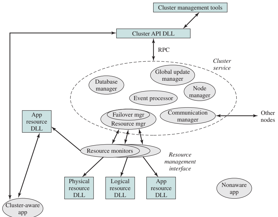
Figure 16.17 Windows Cluster Server Block Diagram
