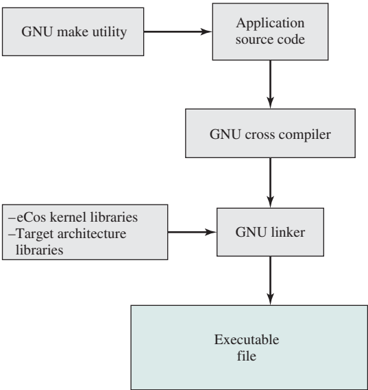
Figure 13.4 Loading an eCos Configuration
