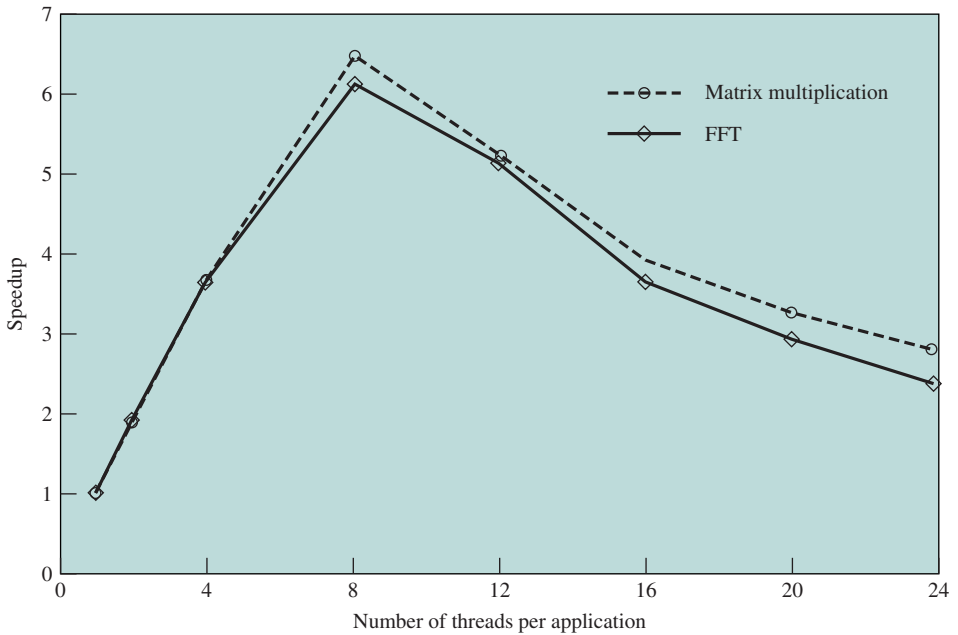
Figure 10.3 Application Speedup as a Function of Number of Threads [TUCK89]
