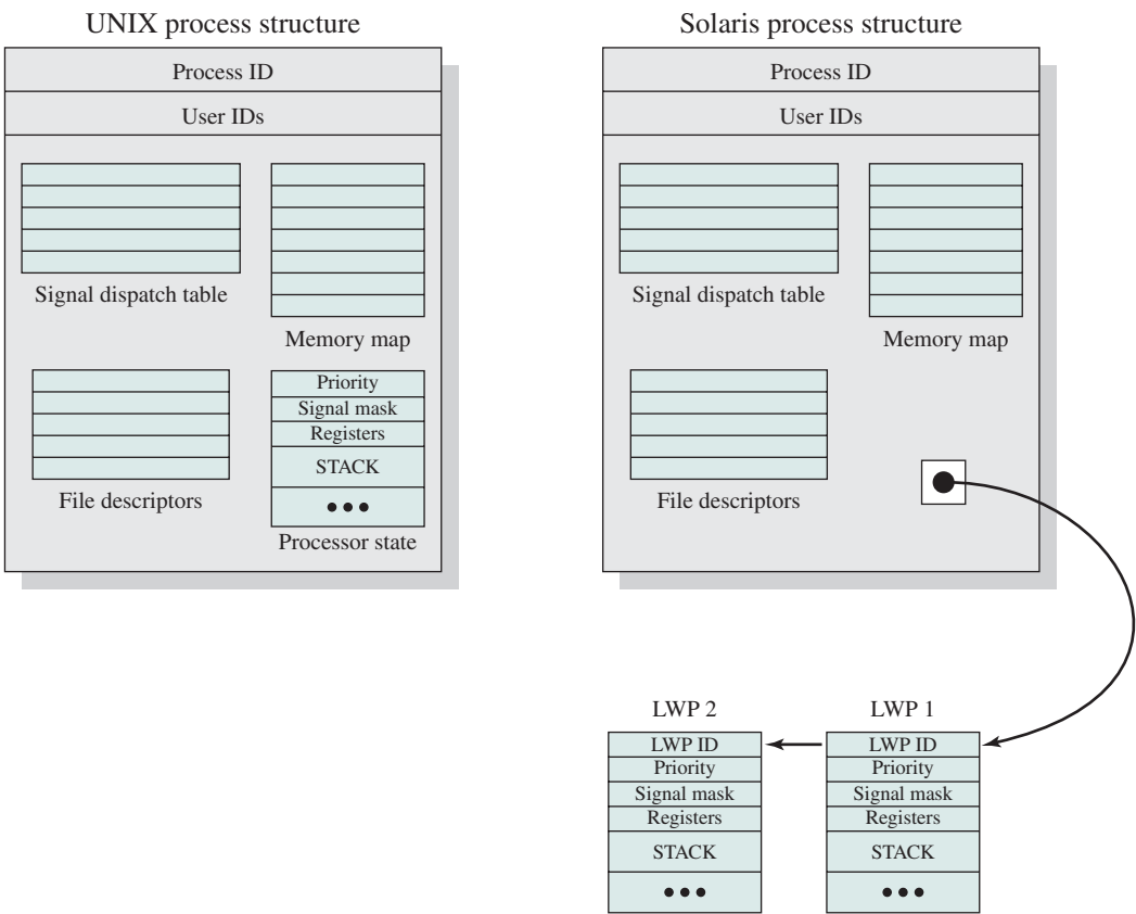
Figure 4.14 Process Structure in Traditional UNIX and Solaris [LEWI96]
