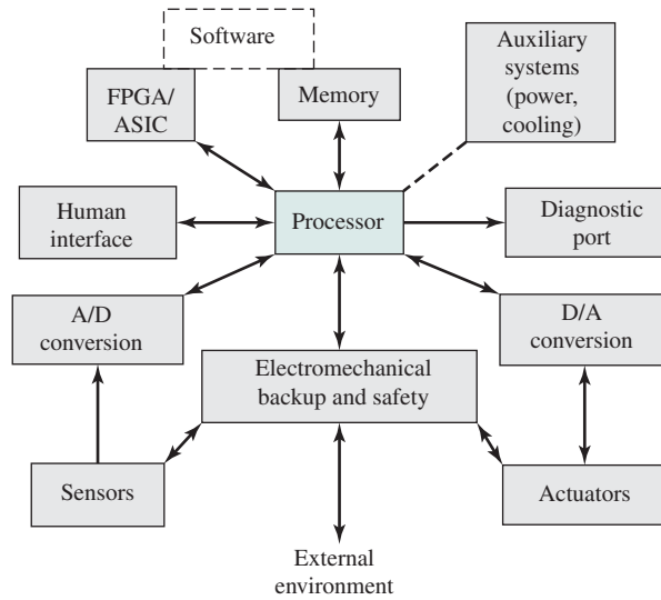
Figure 13.1 Possible Organization of an Embedded System
