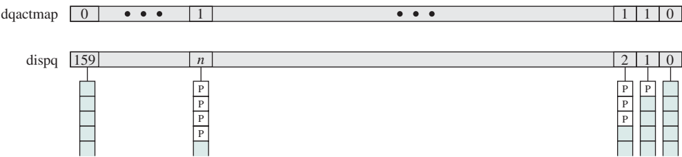
Figure 10.13 SVR4 Dispatch Queues
