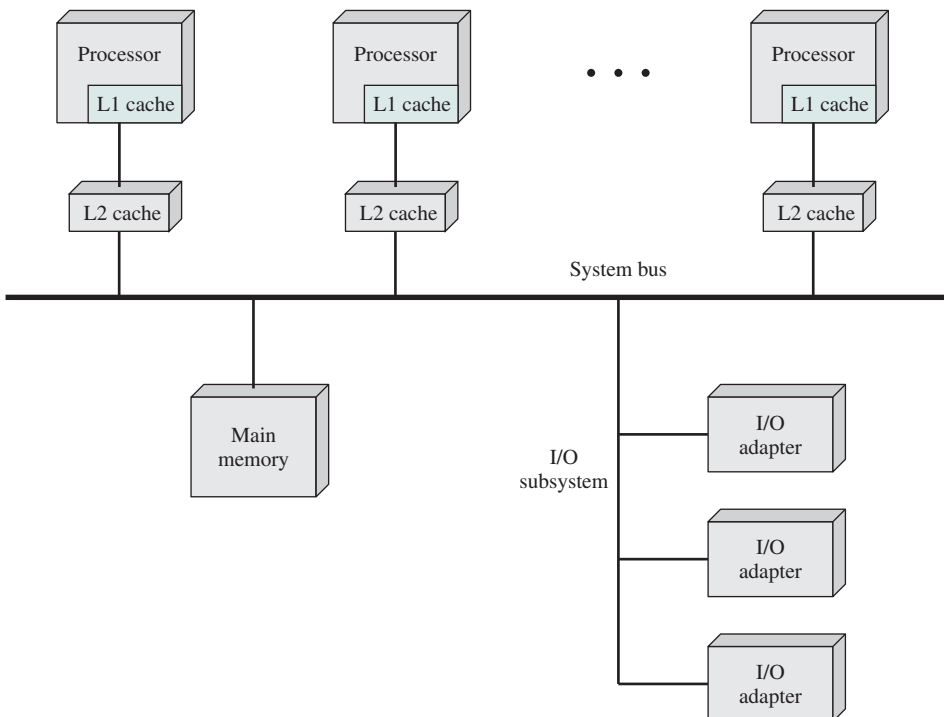
Figure 1.19 Symmetric Multiprocessor Organization
