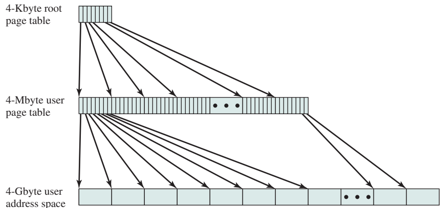
Figure 8.4 A Two-Level Hierarchical Page Table
