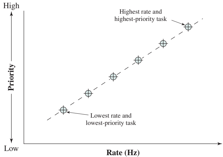
Figure 10.7 A Task Set with RMS [WARR91]
