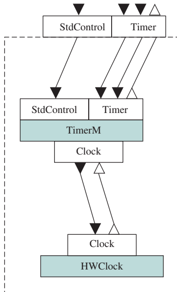
(b) TimerC configuration
