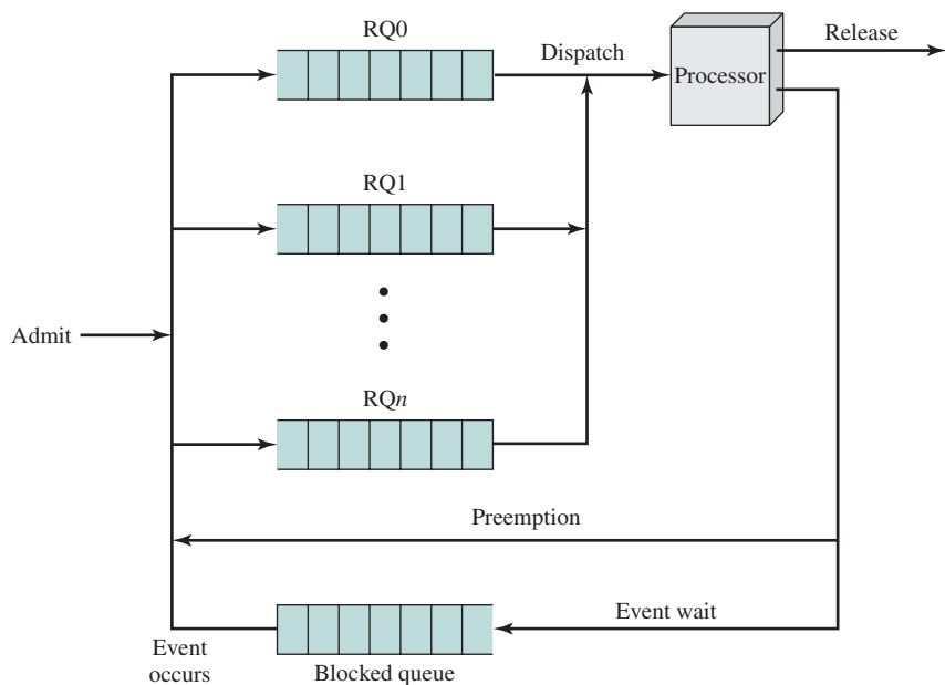
Figure 9.4 Priority Queueing
