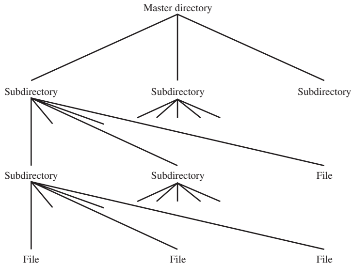
Figure 12.6 Tree-Structured Directory
