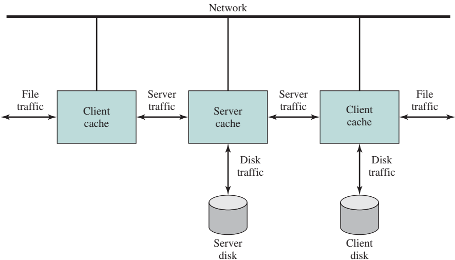
Figure 16.7 Distributed File Cacheing in Sprite
