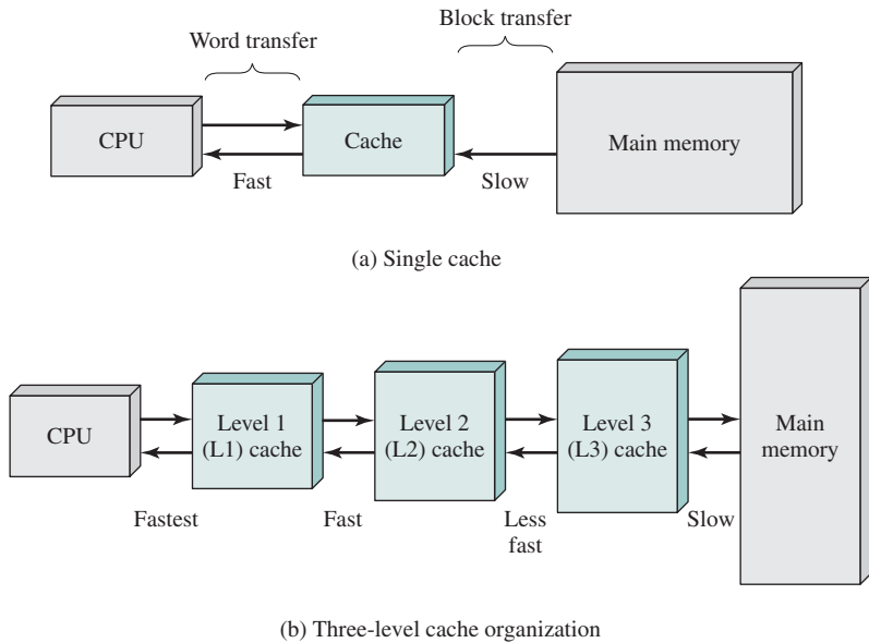
Figure 1.16 Cache and Main Memory
