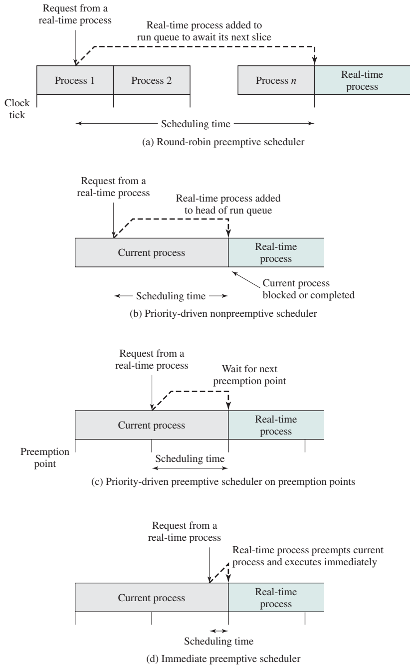
Figure 10.4 Scheduling of Real-Time Process
