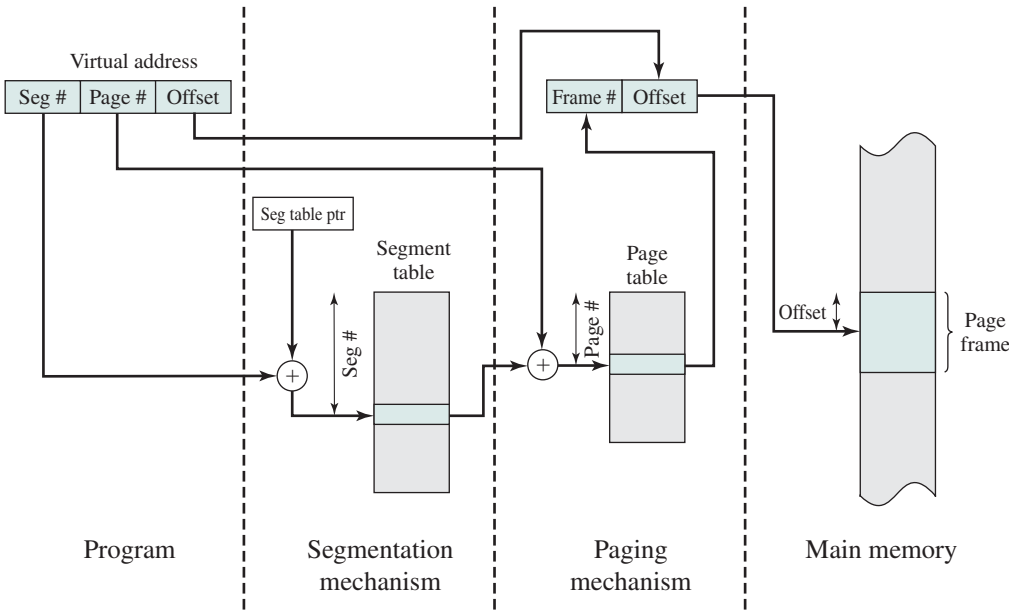
Figure 8.13 Address Translation in a Segmentation/Paging System
