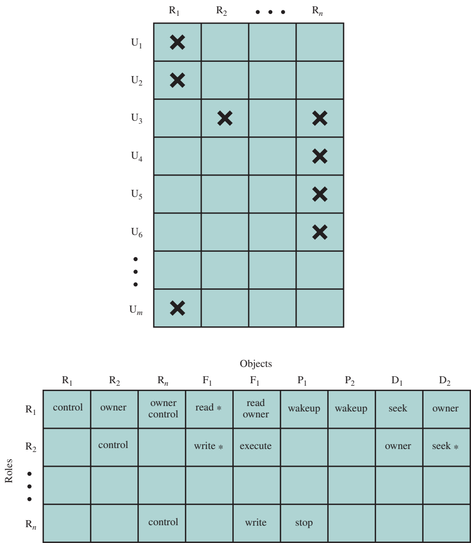
Figure 15.7 Access Control Matrix Representation of RBAC
