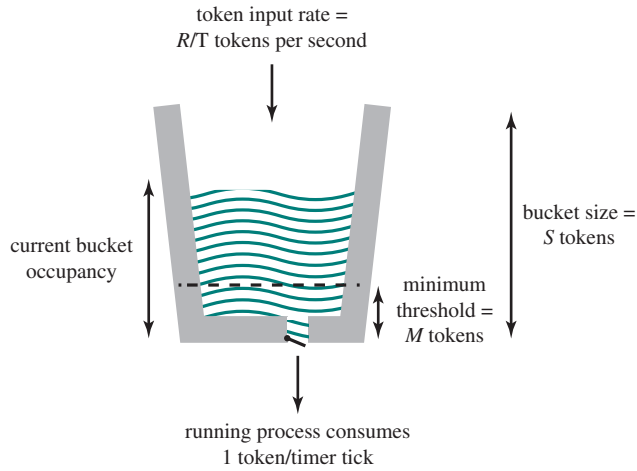
Figure 10.16 Linux VServer Token Bucket Scheme
