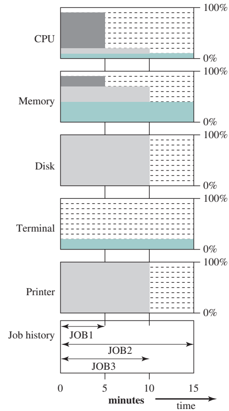
(b) Multiprogramming
