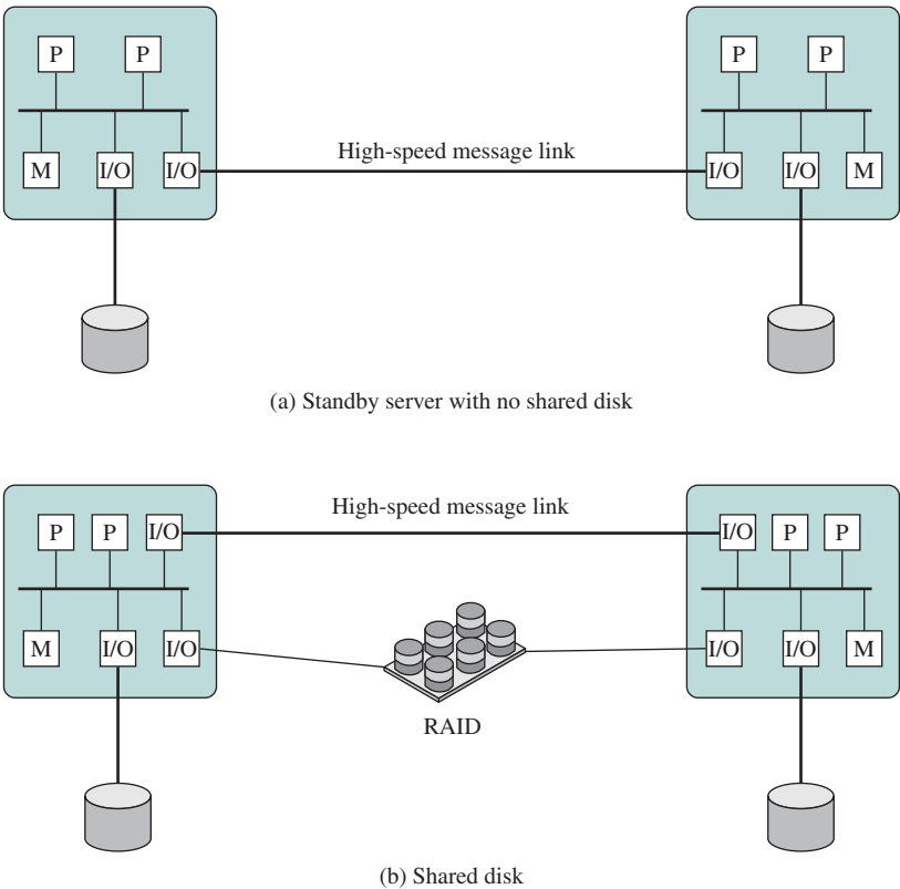
Figure 16.15 Cluster Configurations
