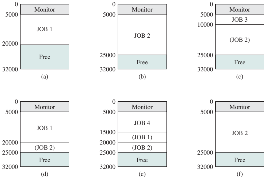
Figure 2.7 CTSS Operation
