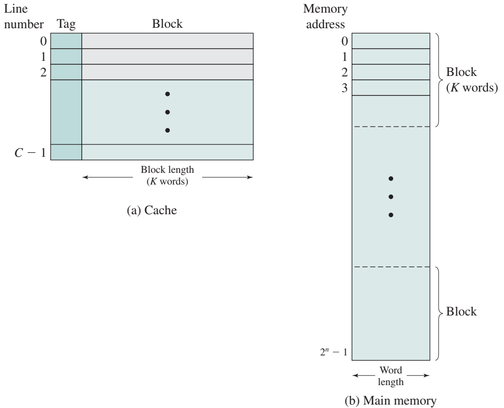
Figure 1.17 Cache/Main-Memory Structure
