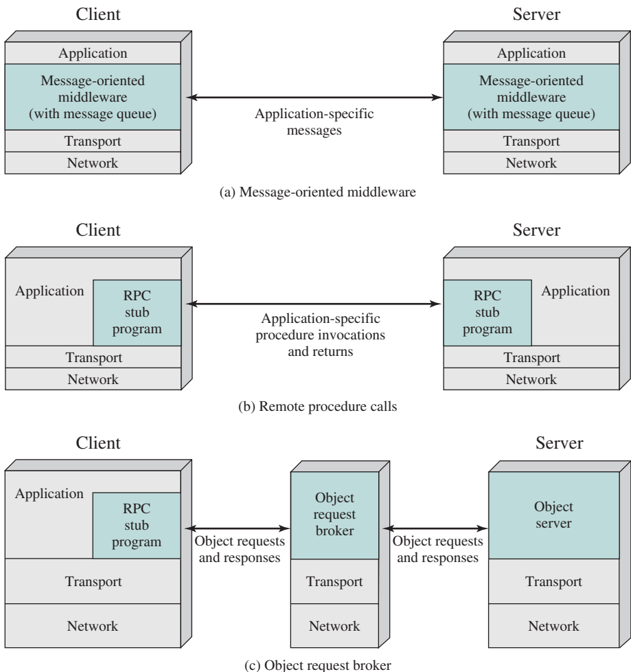
Figure 16.12 Middleware Mechanisms
