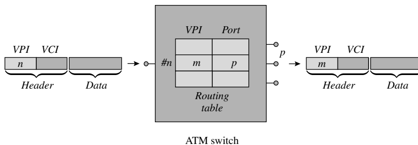
Figure 16.9 An ATM switch.
