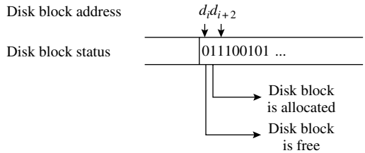
Figure 13.12 Disk status map (DSM).
