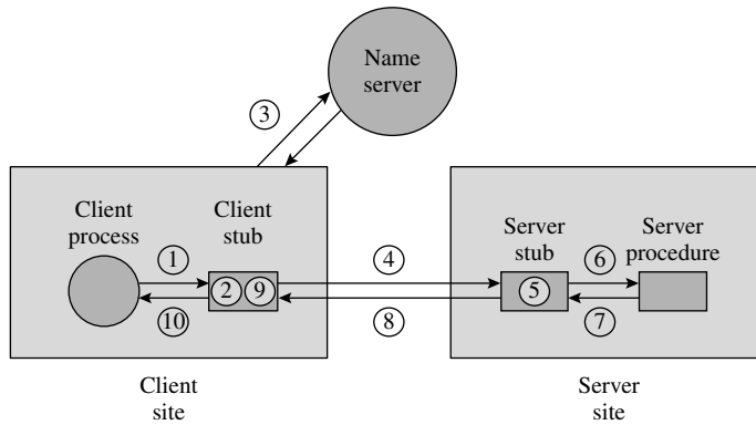
Figure 16.6 Implementation of a remote procedure call (RPC).
