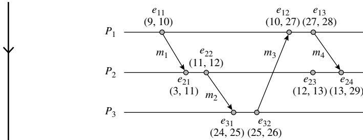
Figure 17.3 Synchronization of logical clocks.
