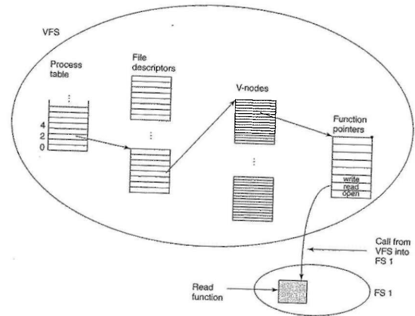
FIG. 4-19. Structures and code used by the VFS and concrete file system to do a read.
