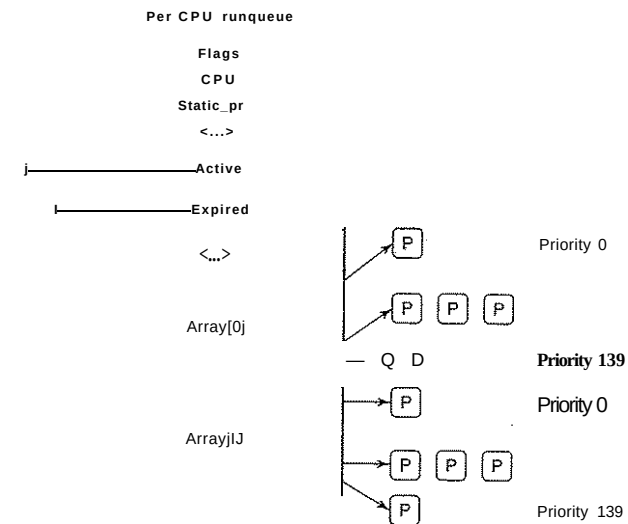
Figure 10-10. Illustration of Linux runqueue and priority arrays.
