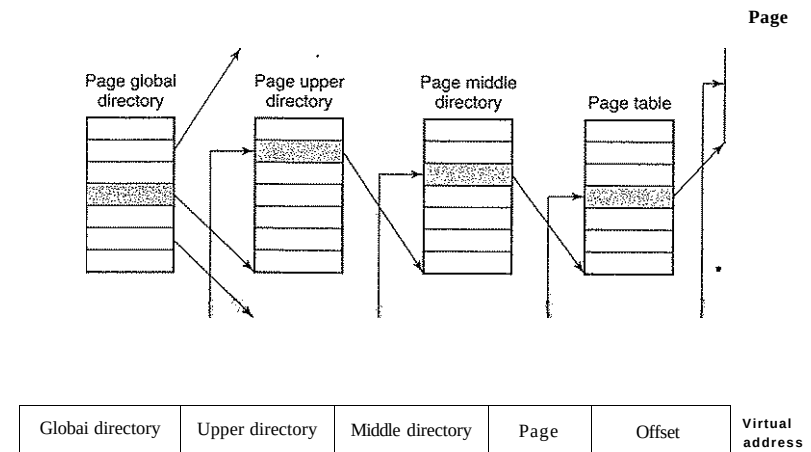
Figure 10-16. Linux uses four-level page tables.
