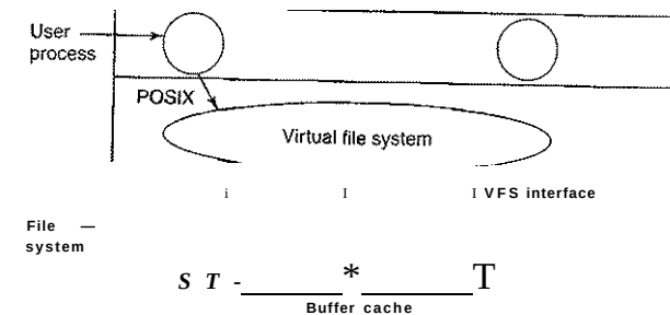
Figure 4-18. Position of the virtual file system.
