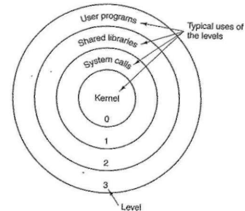
Figure 3-43. Protection on the Pentium.
