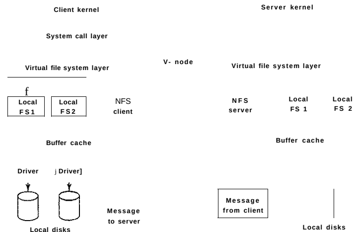
Figure 10-36. The NFS layer structure
