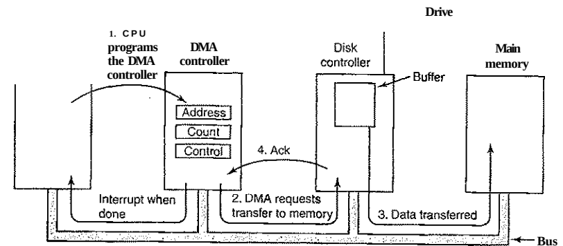
Figure 5-4. Operation of a DMA transfer.
