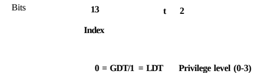
Figure 3-39. A Pentium selector.
