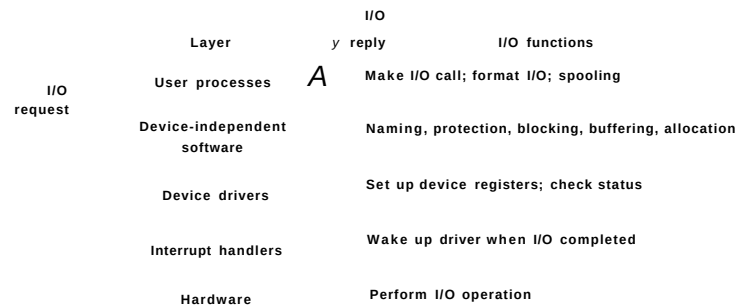
Figure 5-17. Layers of the I/O system and the main functions of each layer.
