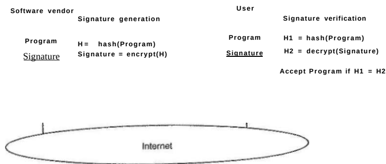
Figure 9-34. How code signing works.
