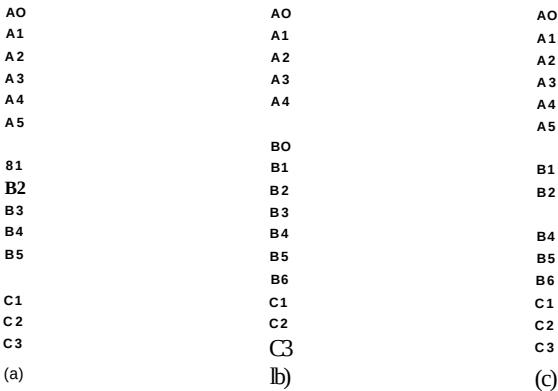
Figure 3-23. Local versus global page replacement, (a) Original configuration, (b) Local page replacement, (c) Global page replacement.
