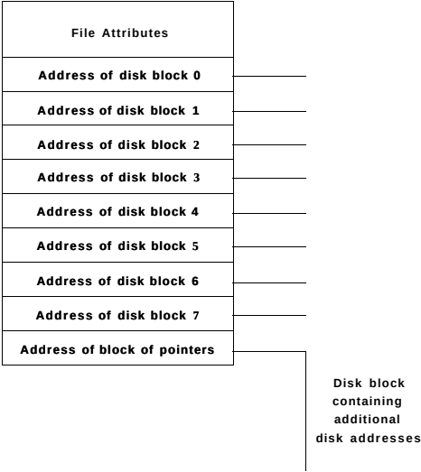
Figure 4-13. An example i-node.
