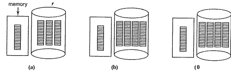
Figure 4-23. (a) An almost-full block of pointers to free disk blocks in memory and three blocks of pointers on disk, (b) Result of freeing a three-block file, (c) An alternative strategy for handling the three free blocks. The shaded entries represent pointers to free disk blocks.
