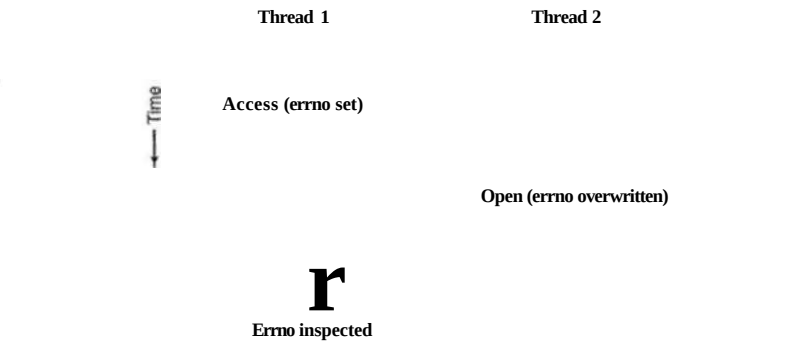
Figure 2-19. Conflicts between threads over the use of a global variable.
