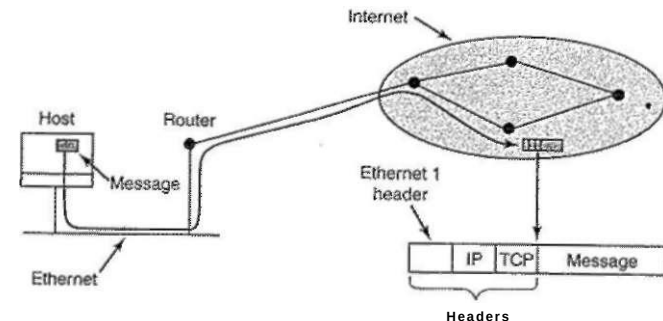
Figure 8-34. Accumulation of packet headers.
