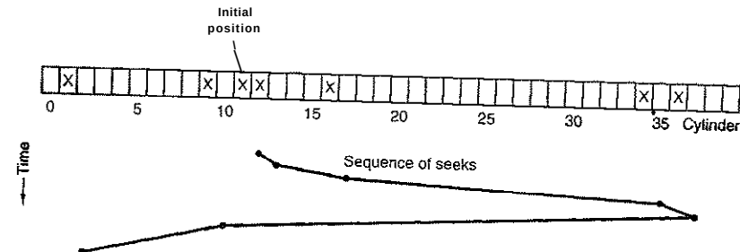
Figure 5-29. The elevator algorithm for scheduling disk requests.
