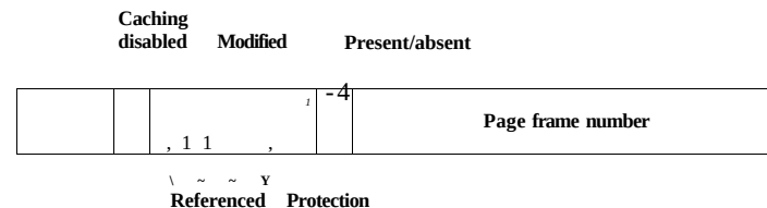
Figure 3-11. A typical page table entry.
