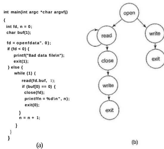
Figure 9-36. (a) A program, (b) System call graph for (a).
