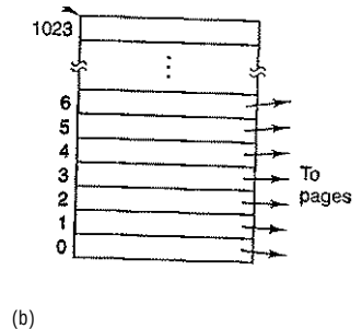
Figure 3-13. (a) A 32-bit address with two page table fields, (b) Two-level page tables.
