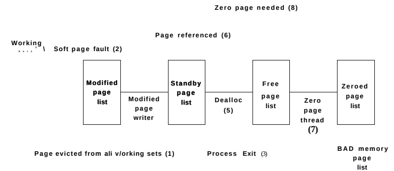
Figure 11-36. The various page lists and the transitions between them.
