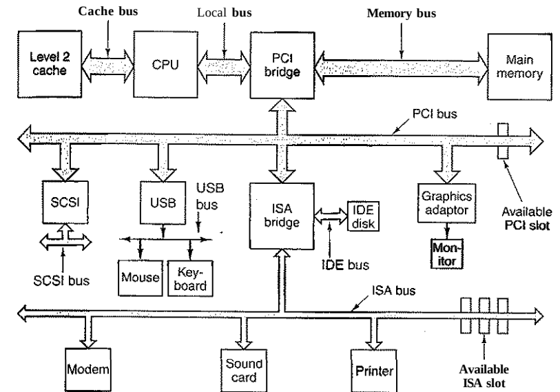
Figure 1-12. The structure of a large Pentium system
