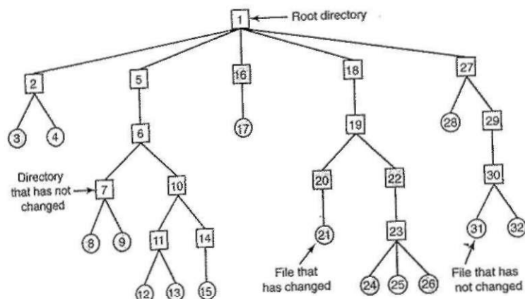
Figure 4-26(a) A file system to be dumped. The squares are directories and the circles are files. The shaded items have been modified since the last dump. Each directory and file is labeled by its i-node number.
