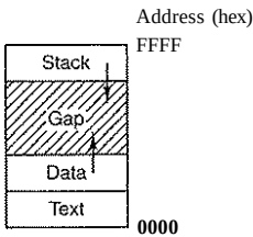
Figure 1-20- Processes have three segments: text, data, and stack.
