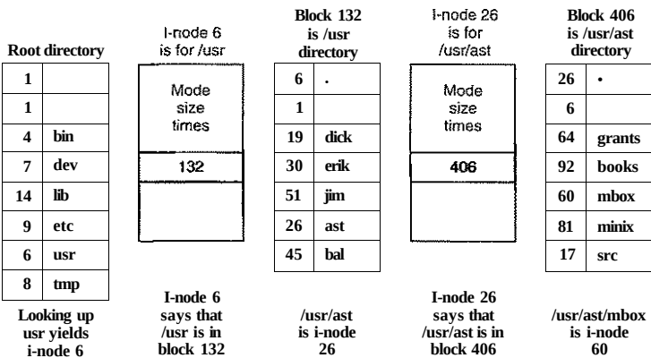
Figure 4-35. The steps in looking up /usr/ast/mbox .
