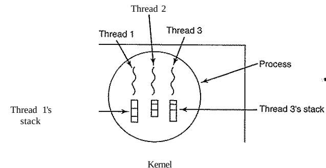
Figure 2-13. Each thread has its own stack.
