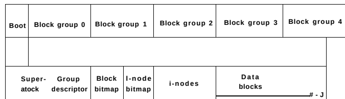
Figure 10-31. Disk layout of the Linux ext2 file system.
