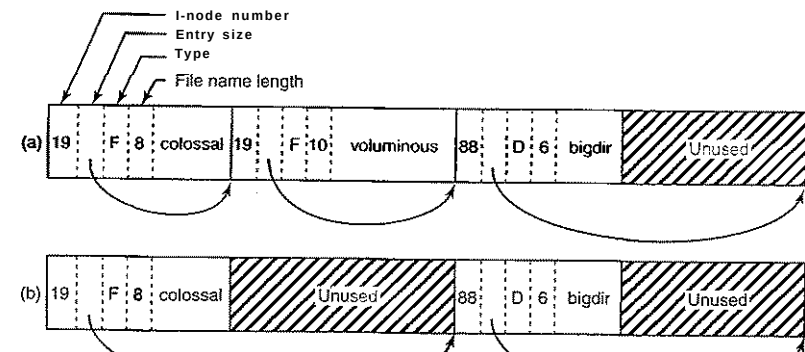
Figure 10-32. (a) A Linux directory with three files, (b) The same directory after the file voluminous has been removed.
