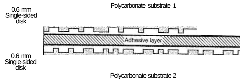
Figure 5-24. A double-sided, dual-layer DVD disk.
